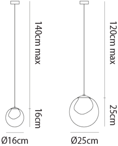
Product Dimensions
