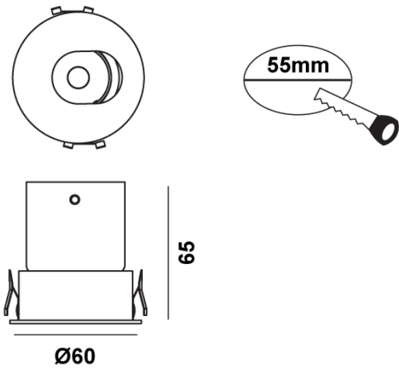
Product Dimensions
