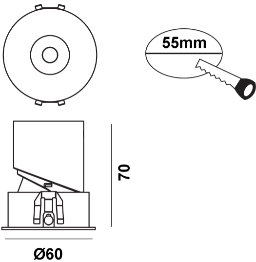
Product Dimensions
