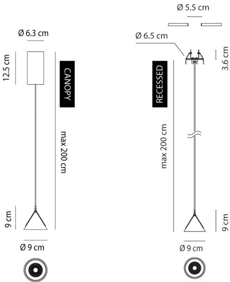
Product Dimensions
