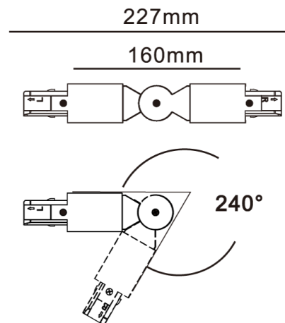
Product Dimensions
