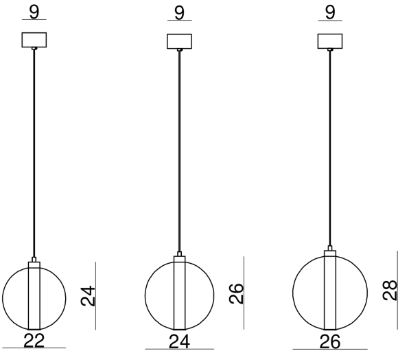
Product Dimensions
