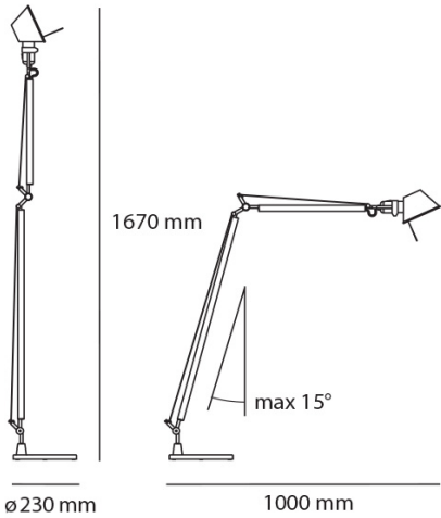
Product Dimensions
