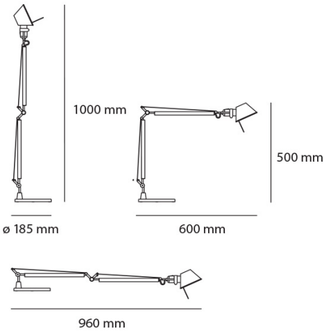
Product Dimensions
