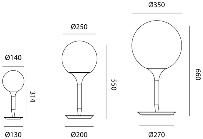
Product Dimensions
