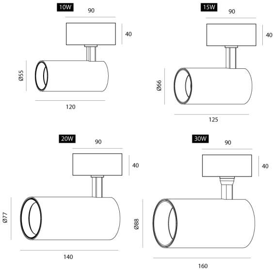
Product Dimensions
