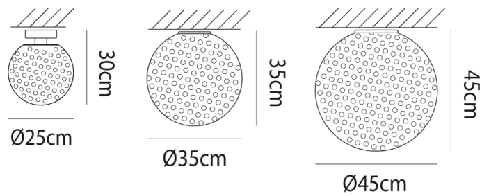
Product Dimensions
