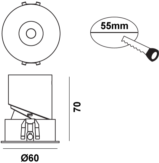
Product Dimensions
