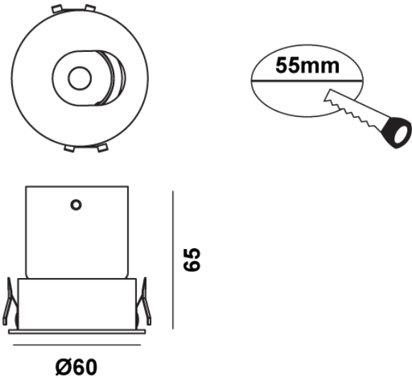
Product Dimensions
