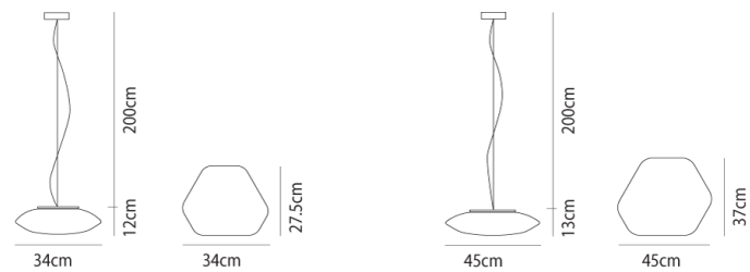
Product Dimensions
