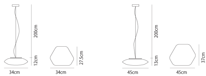
Product Dimensions
