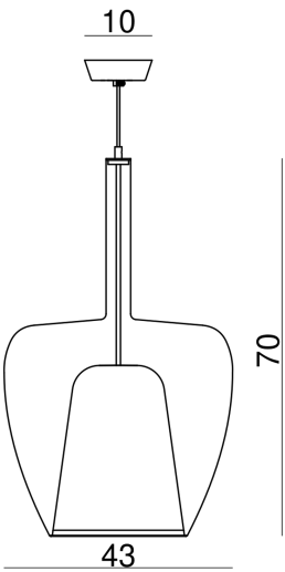
Product Dimensions
