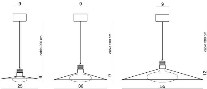
Product Dimensions
