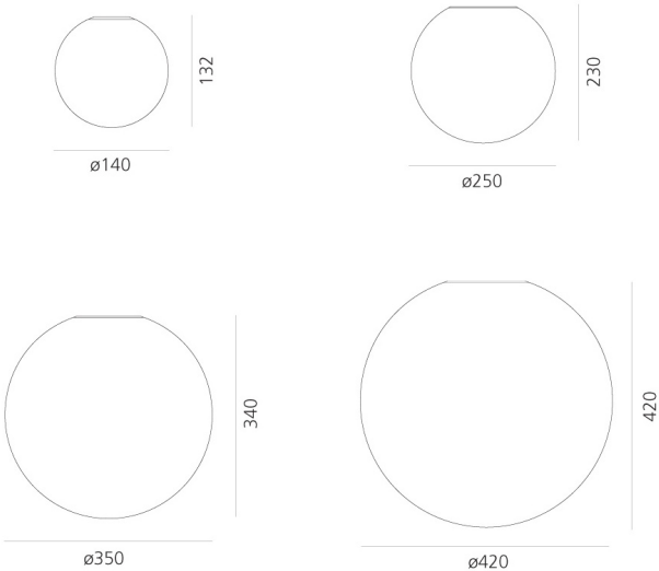
Product Dimensions
