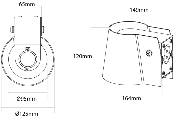
Product Dimensions
