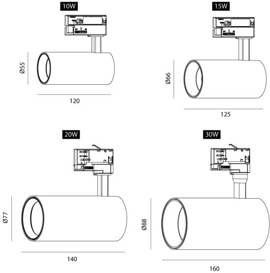
Product Dimensions
