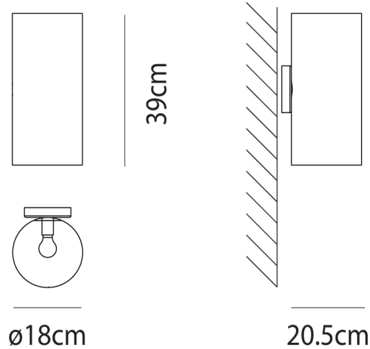
Product Dimensions
