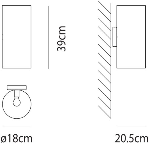
Product Dimensions
