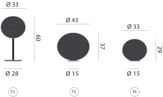
Product Dimensions
