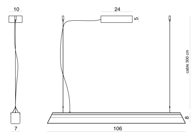
Product Dimensions
