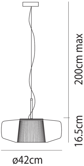
Product Dimensions
