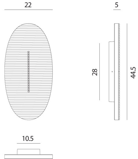
Product Dimensions
