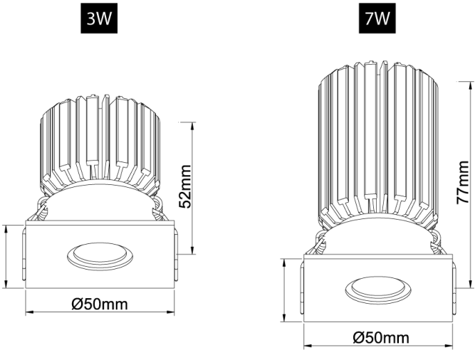
Cut Out: Ø45mm
