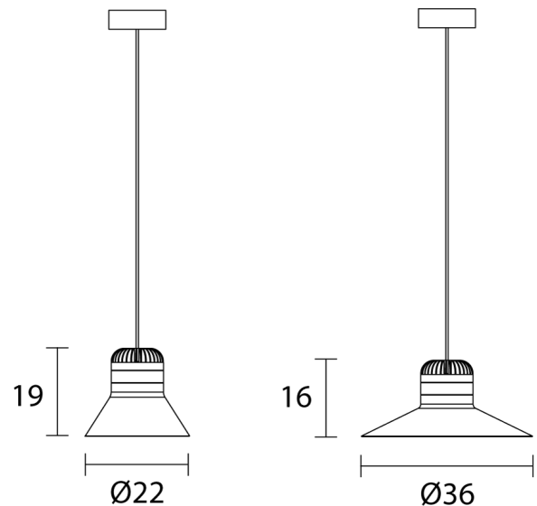
Product Dimensions
