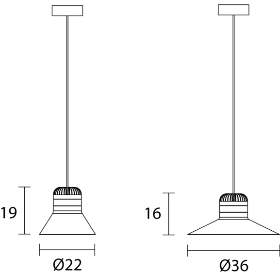
Product Dimensions
