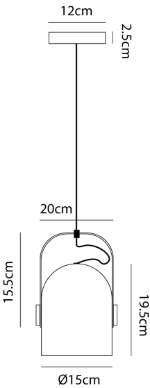
Product Dimensions
