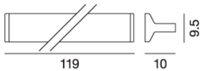
Product Dimensions
