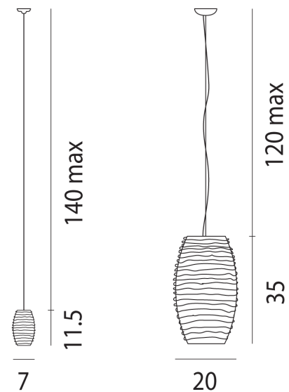
Product Dimensions
