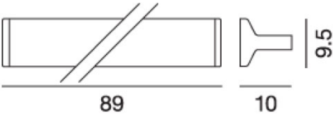
Product Dimensions
