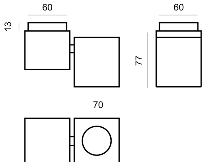
Product Dimensions
