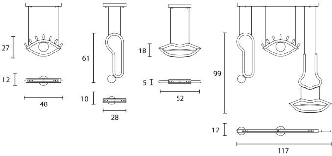
Product Dimensions
