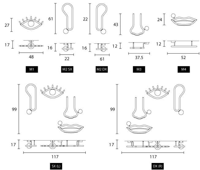
Product Dimensions
