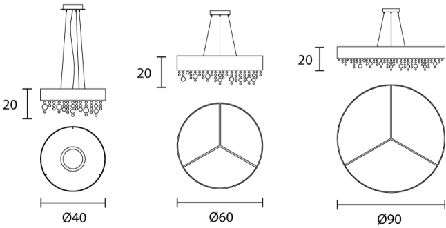
Product Dimensions
