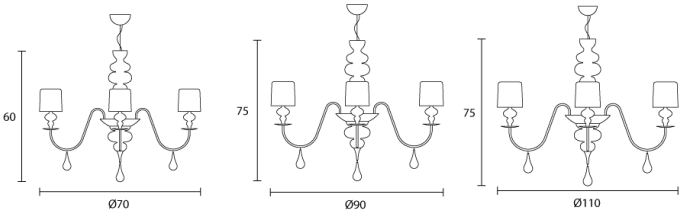
Product Dimensions
