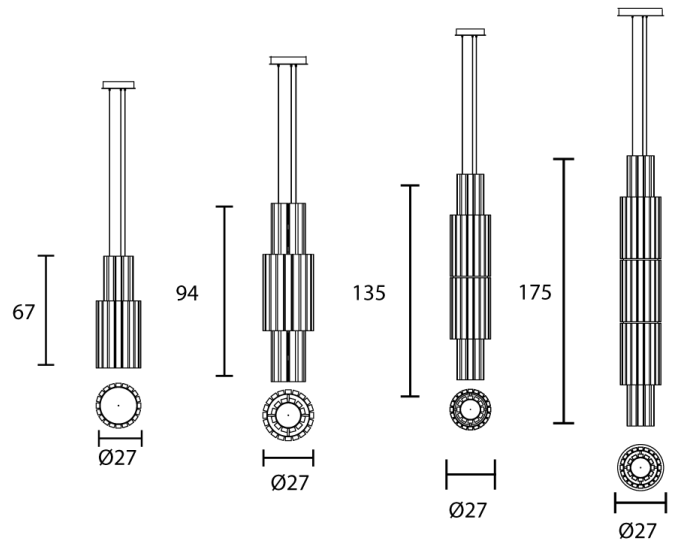
Product Dimensions
