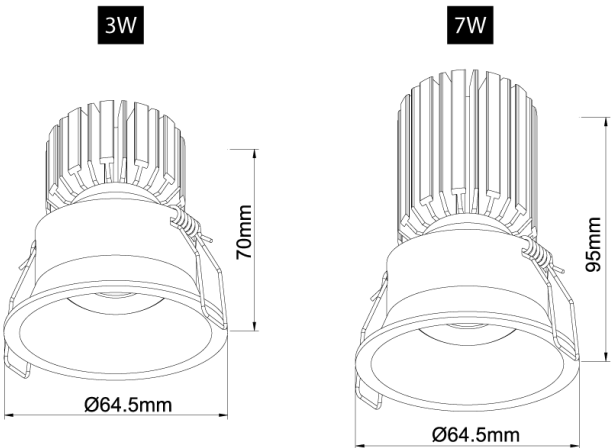
Cut Out: Ø58mm
