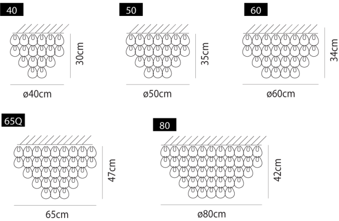
Product Dimensions
