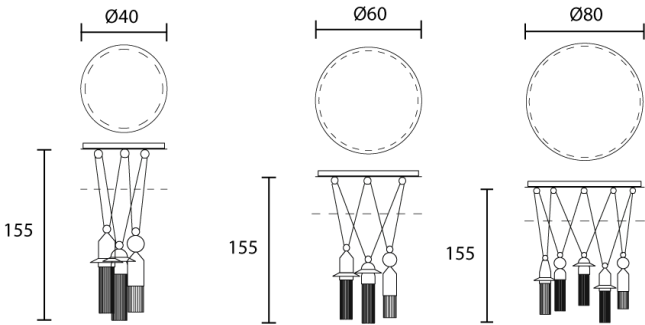
Product Dimensions
