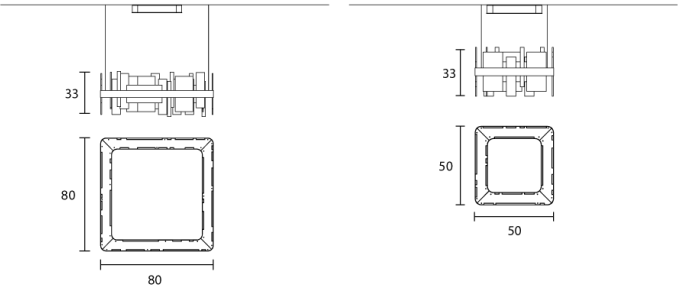
Product Dimensions
