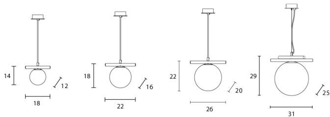
Product Dimensions
