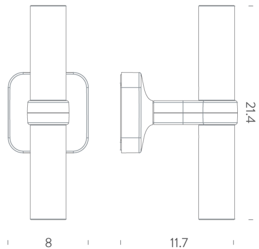
Product Dimensions
