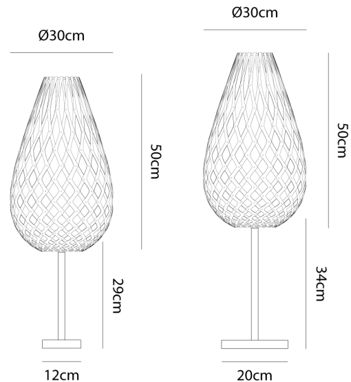
Product Dimensions
