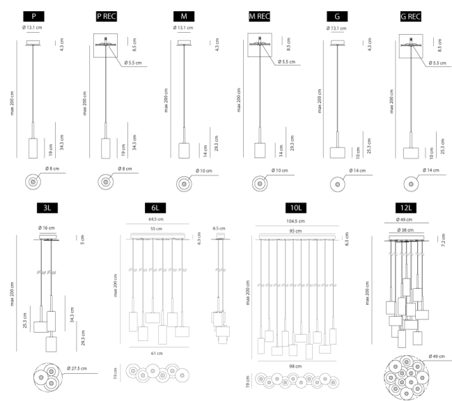
Product Dimensions
