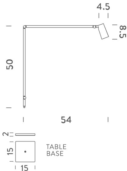
Product Dimensions
