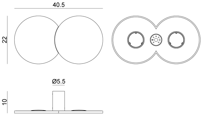
Product Dimensions
