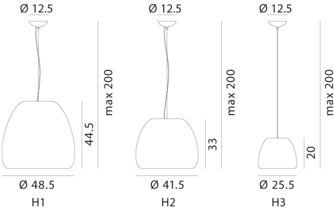
Product Dimensions
