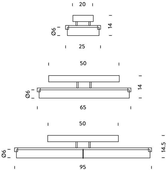
Product Dimensions
