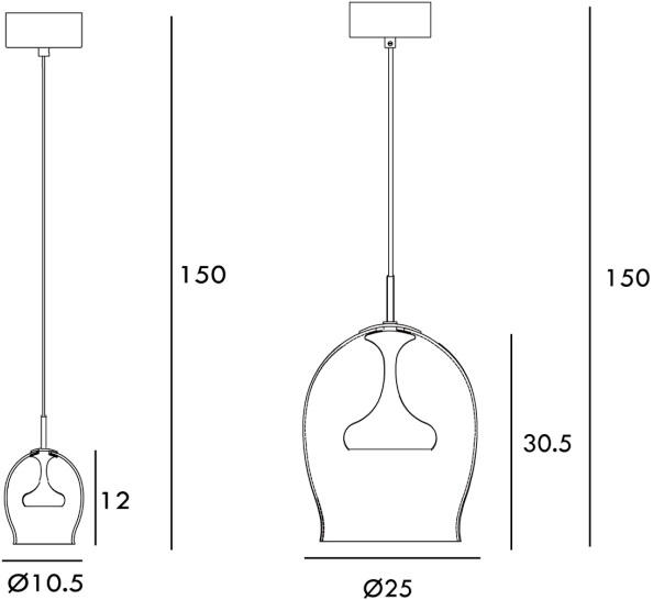
Product Dimensions
