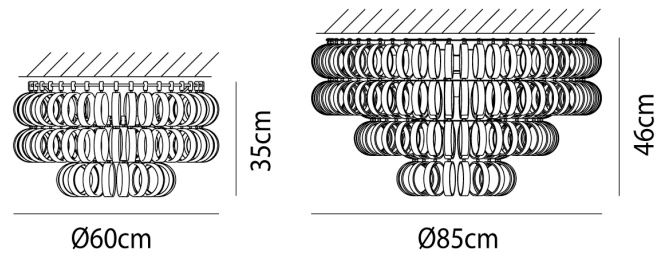
Product Dimensions
